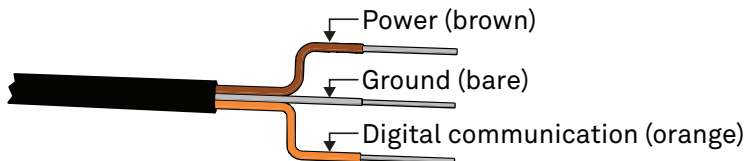
Figure 9 Pigtail wiring
